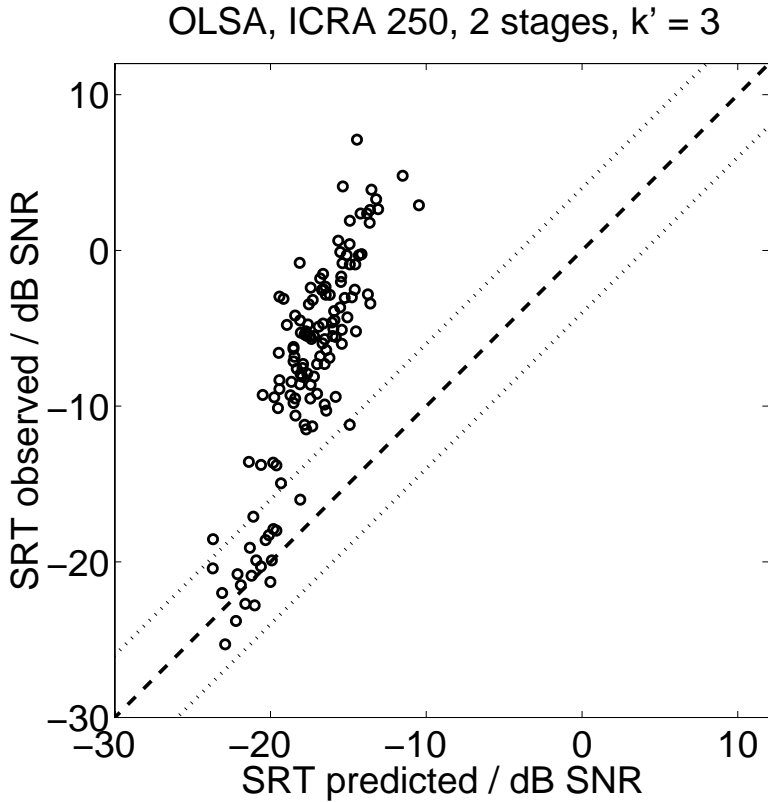
Figure 7.8: Intelligibility predictions for icra5-250 noise by two-stage speech perception model, k' = 3 . Each circle indicates one pair of observed/predicted SRT. The dashed lines indicate the estimated 95%-confidence interval of the observed data.
