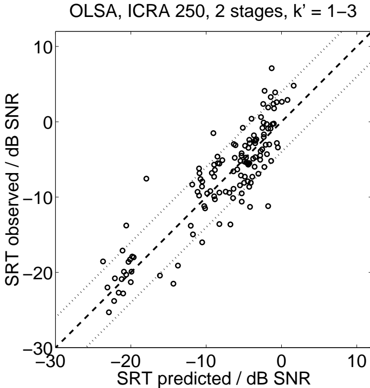
Figure 7.9: Intelligibility predictions for icra5-250 noise by two-stage speech perception model with integrated context concept and three different k' values. Each circle indicates one pair of observed/predicted SRT. The dashed lines indicate the estimated 95%–confidence interval of the observed data.
