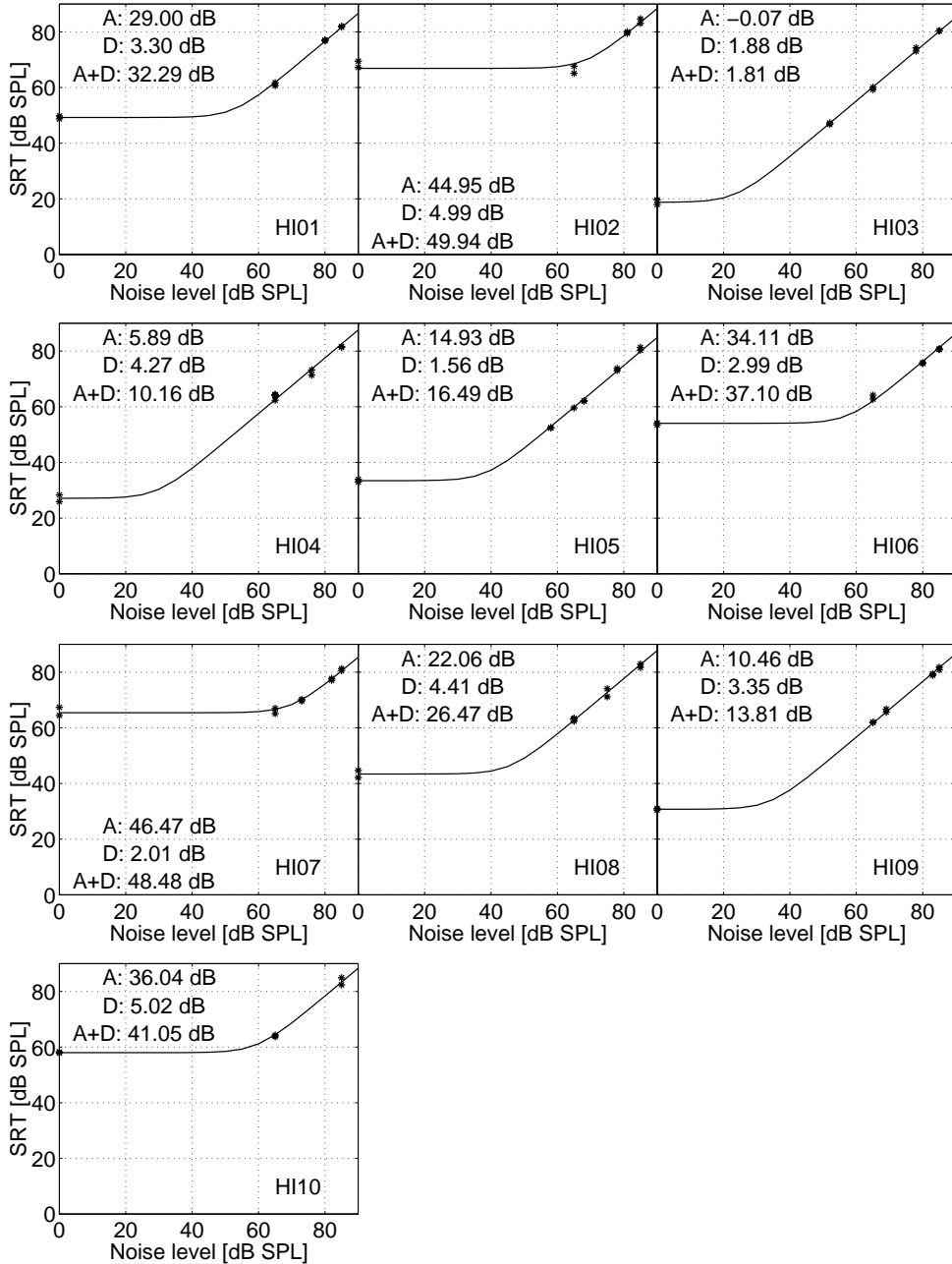
Figure 7.3: Plomp's model function (Equation 7.2) fitted to the Oldenburg sentence test results of 10 hearing-impaired subjects with different types of hearing loss.
