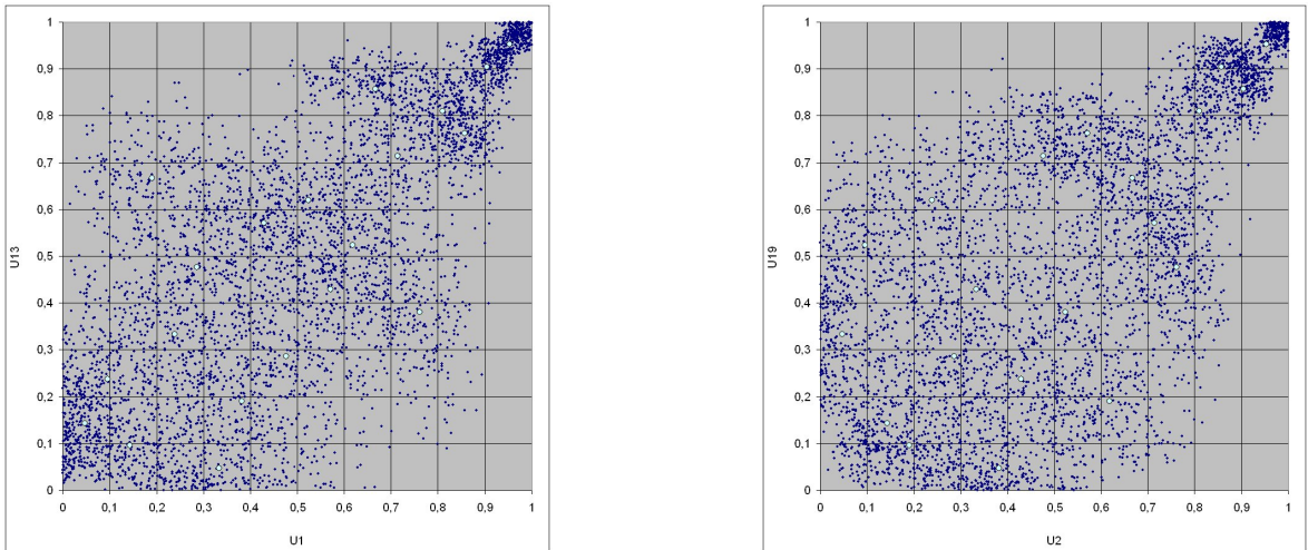
Figure 36: Gamma copula with the rook copula driver, I
