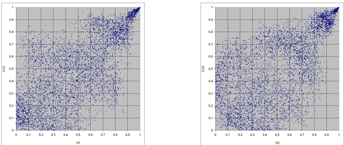
Figure 38: Gamma copula with UF copula driver, I
