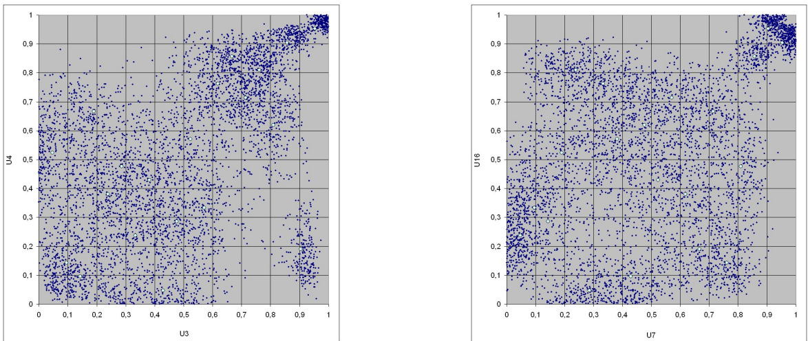
Figure 37: Gamma copula with the rook copula driver, II
