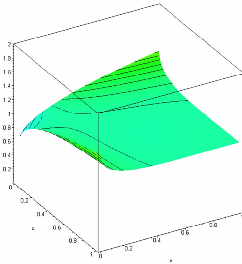
Figure 4: Ratio \frac{c_{a,\text{sing}}^{\text{NB}}(u, v)}{c_{a,\text{sing}}^{\text{G}}(u, v)} , a = 1
