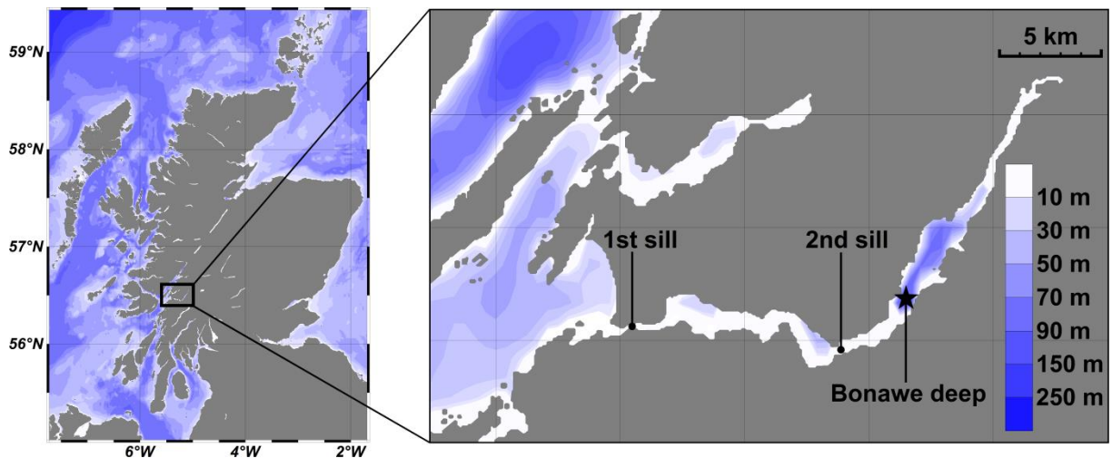
Figure 3.1: Sampling site characteristics. Loch Etive is a sea loch at the western coast of Scotland, UK (56°45'N, 5°18'W). Water exchange with the ocean is limited by two sills. All samplings as well as the mooring deployment were done at the deepest point of the loch, Bonawe deep (~150 m), at the Scottish Association for Marine Science (SAMS) permanent station RE5. Maps were created with Ocean Data View v. 4.7.4 (Schlitzer 2015).
