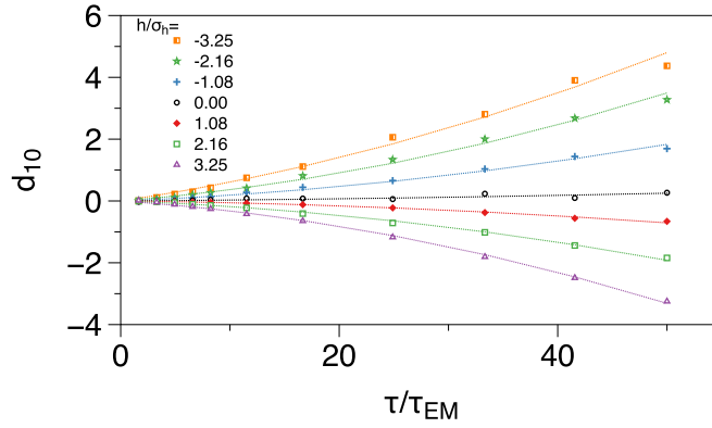
Figure 4. Coefficient d_{10} from equation (14) as a function of \tau for different wave surface height values, h^* . The dotted lines are the second order polynomial fits in \tau .
