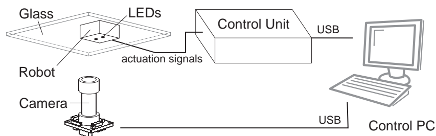
Figure 5.3: Architecture of the tracking system before the FPGA deployment. (Diederichs, 2010)
