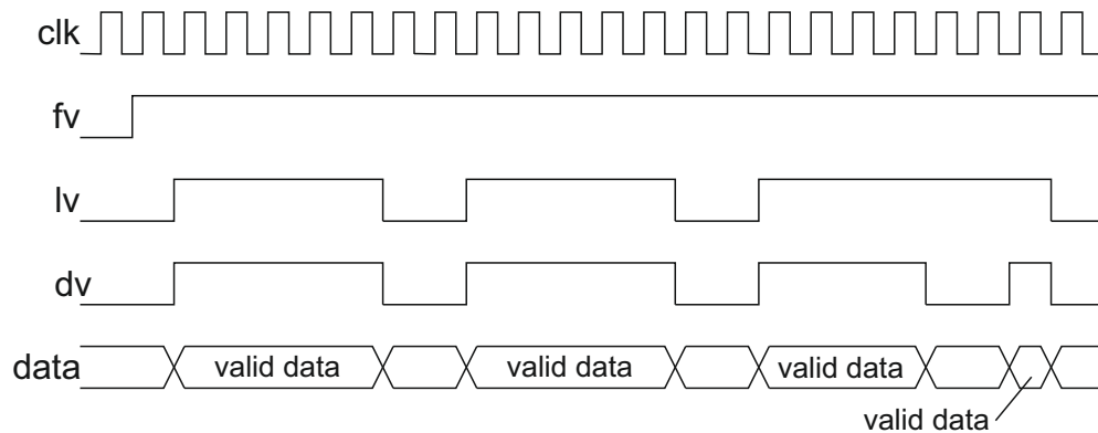
Figure 2.4: Control signals of stream-based image-processing. The general protocol remains the same. The transfer of image data can be interrupted during the transfer of a row. If this happens, the line valid (lv) signal remains high while the data valid (dv) signal changes to low. The pixel value is only valid if the line valid signal and the data valid signal are both high.
