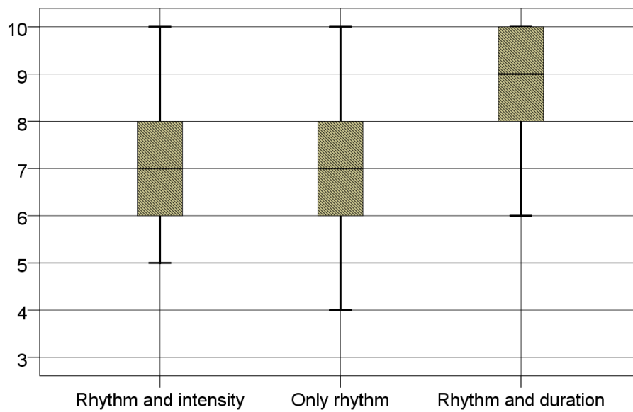
Figure 4.28: Learnability results.
