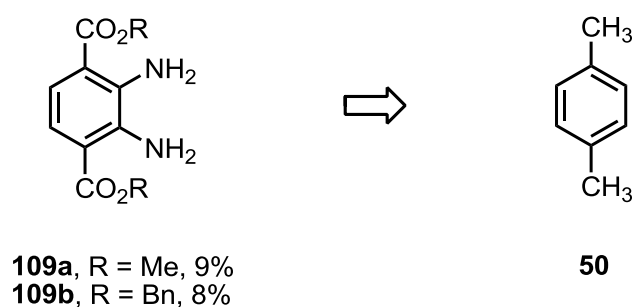
Scheme VI: Retrosynthesis of the dimethyl 2,3-diaminoterephthalates 109a and 109b .
