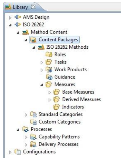
Abbildung 42: Library View
